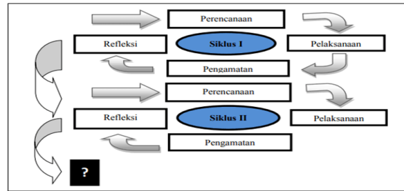
Gambar 1.1 Alur Penelitian
